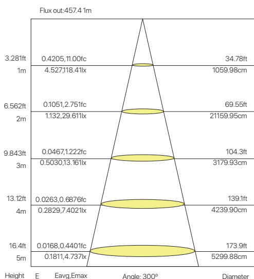
Lux Distance Curve
