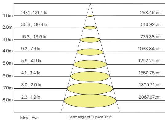
Lux Distance Curve
