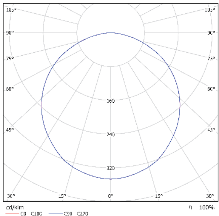
CDL Polar
