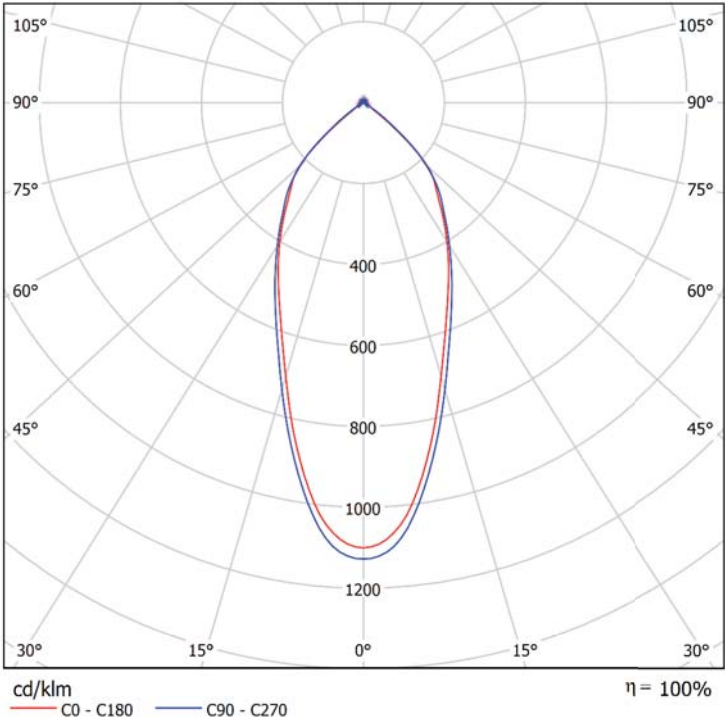
CDL Polar
